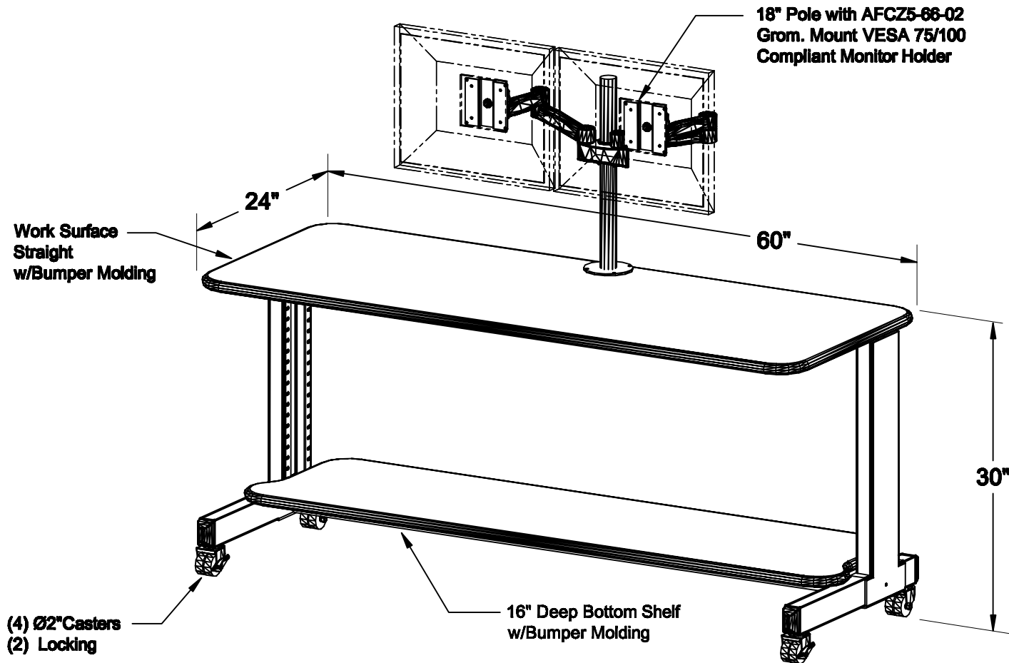
ISOMETRIC VIEW
