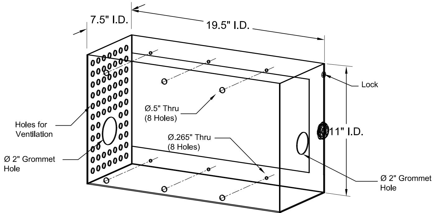
ISOMETRIC VIEW (transparent)
