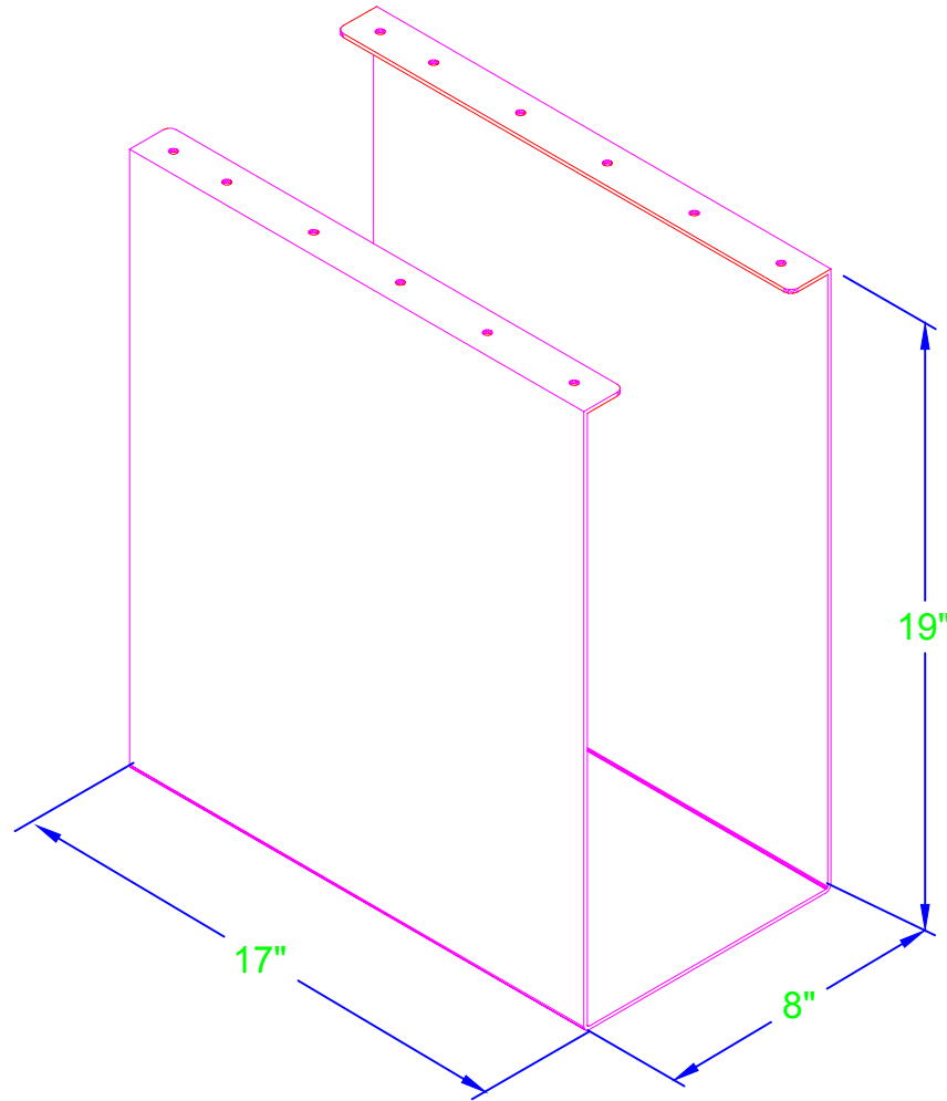
ISOMETRIC VIEW
