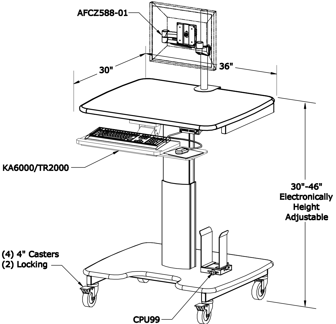
ISOMETRIC VIEW
